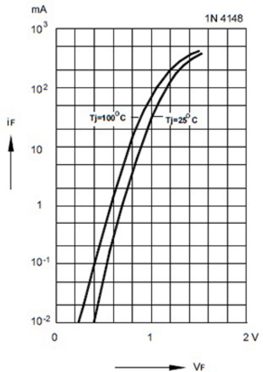
Forward characteristics
